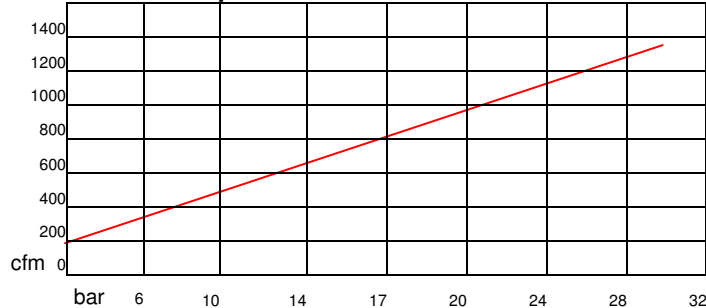
Air Consumption
